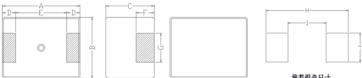
推荐焊盘尺寸 Recommend PC Board Pattern
