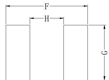
推荐焊盘尺寸 Recommend PC Board Pattern
