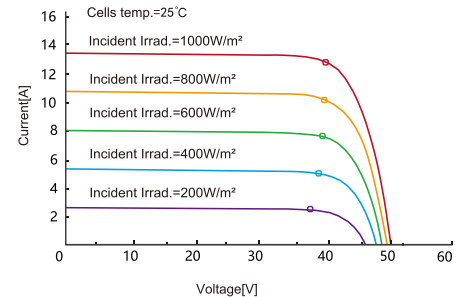
Current-Voltage Curve
