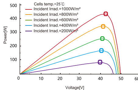
Power-Voltage Curve
