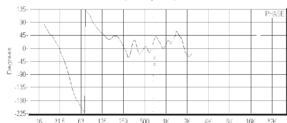
Phase response
