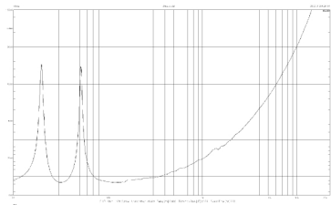
Impedance
