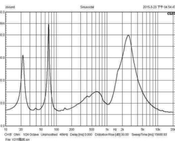
Impedance
