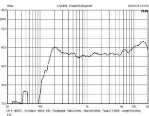
Frequency response
