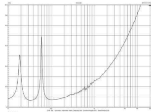
Impedance
