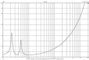
LF Impedance
