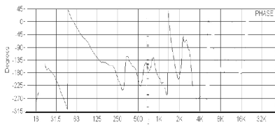
Phase response
