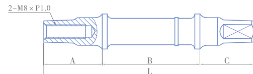
Bolt Type
