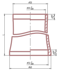
1-1/8"&1-1/4" Semi-Integrated
