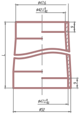
1-1/4" semi-Integrated
