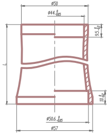
1-1/8"&1-1/4" Semi-Integrated
