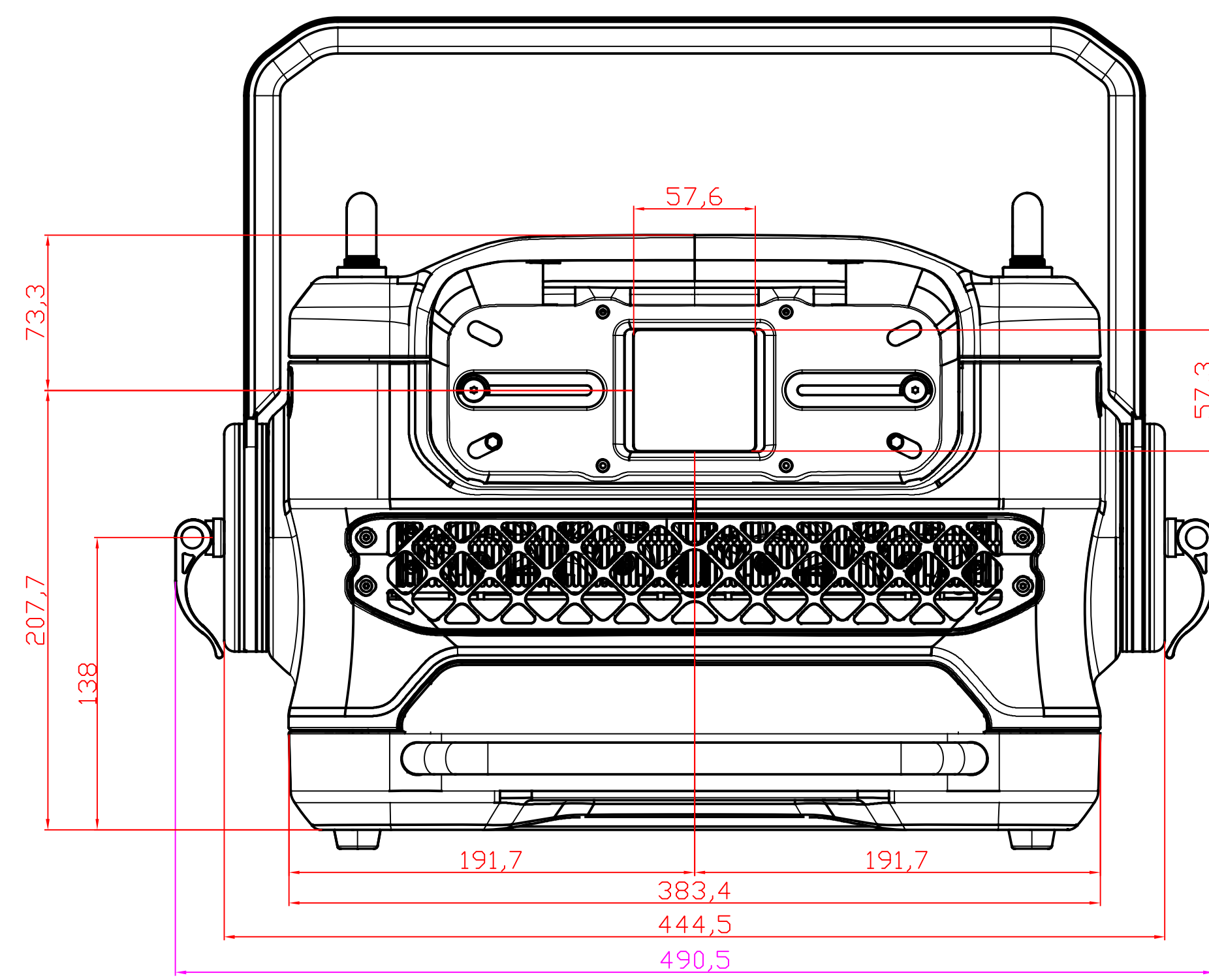
FRONT VIEW
