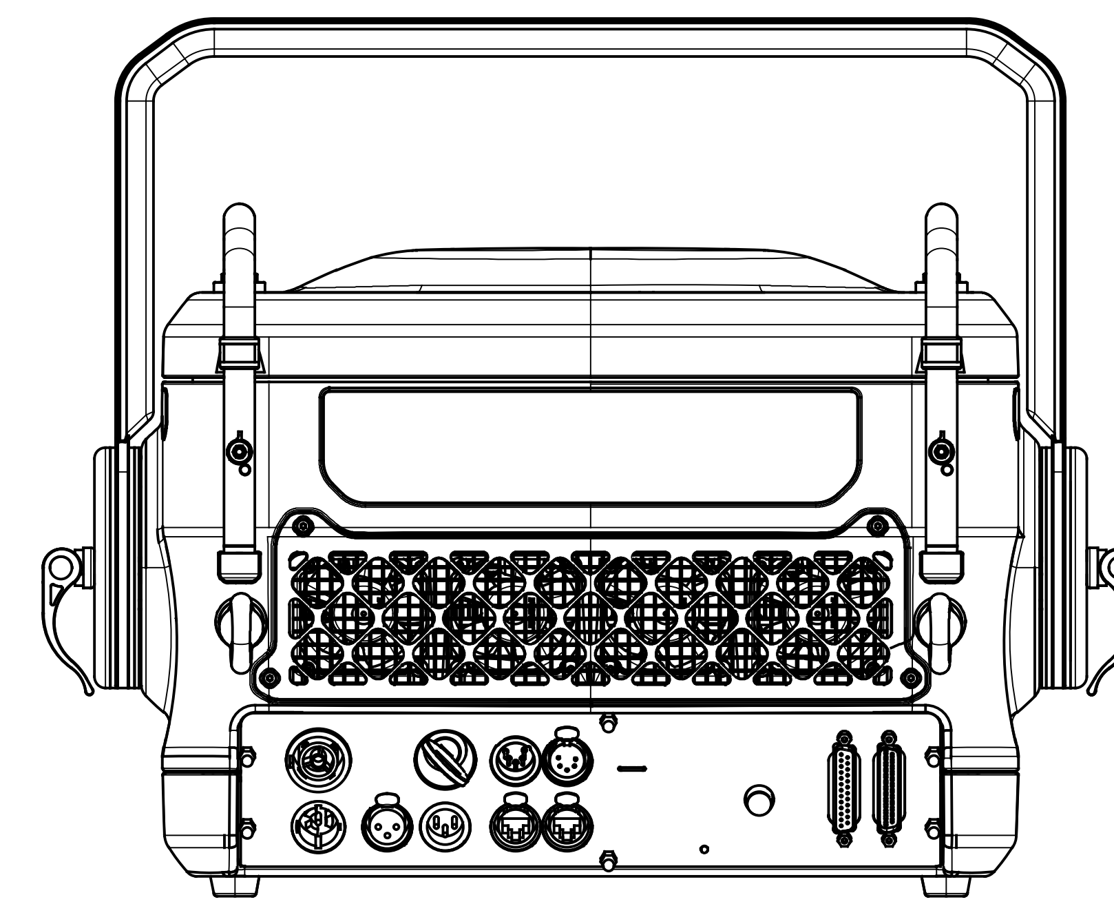
REAR VIEW
