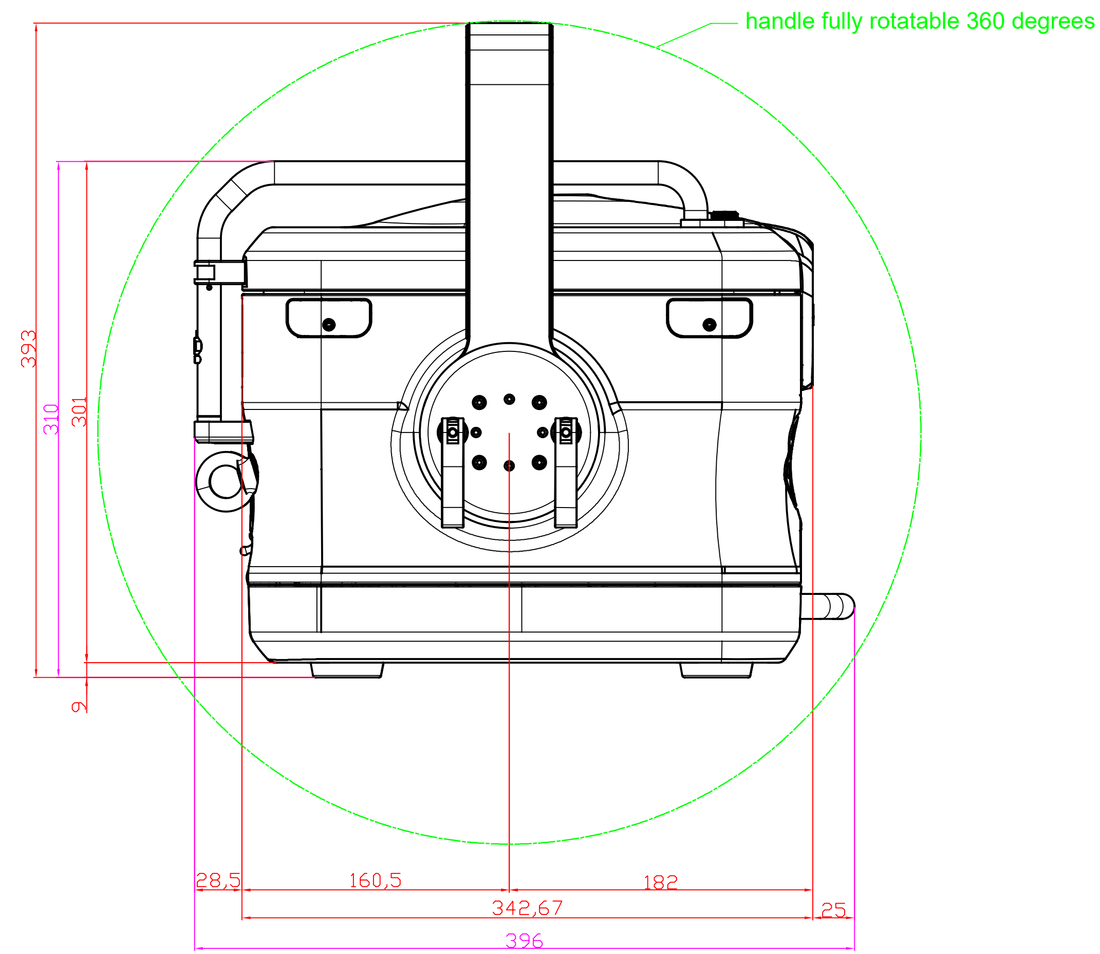
SIDE VIEW
