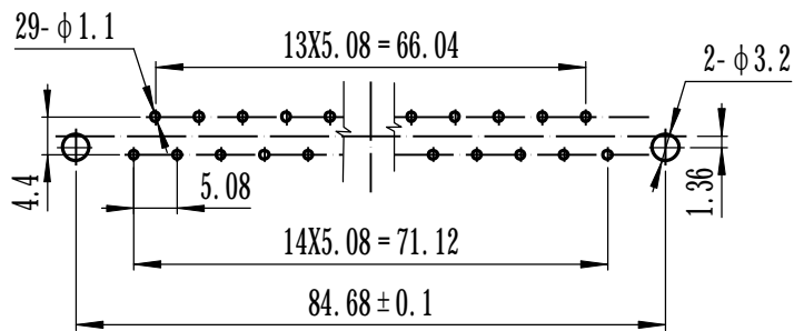
推荐插座安装开孔尺寸
