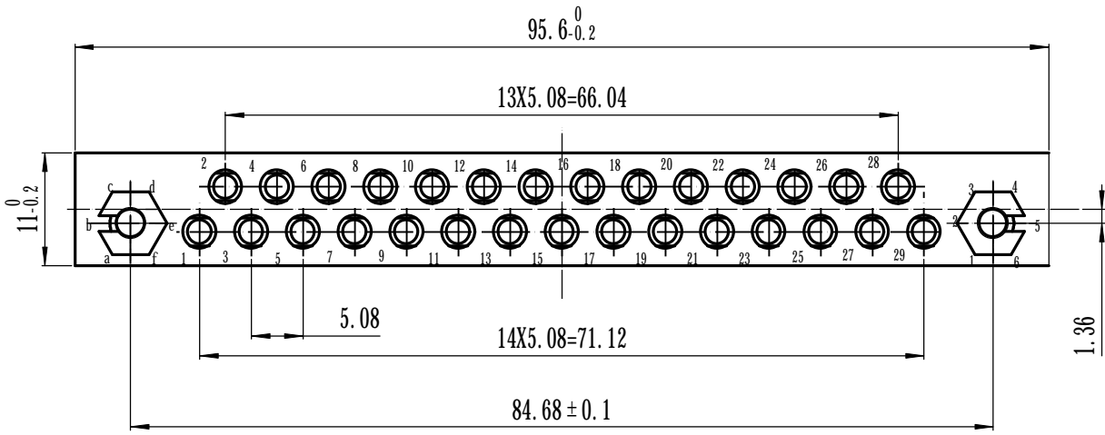
推荐插座安装开孔尺寸
