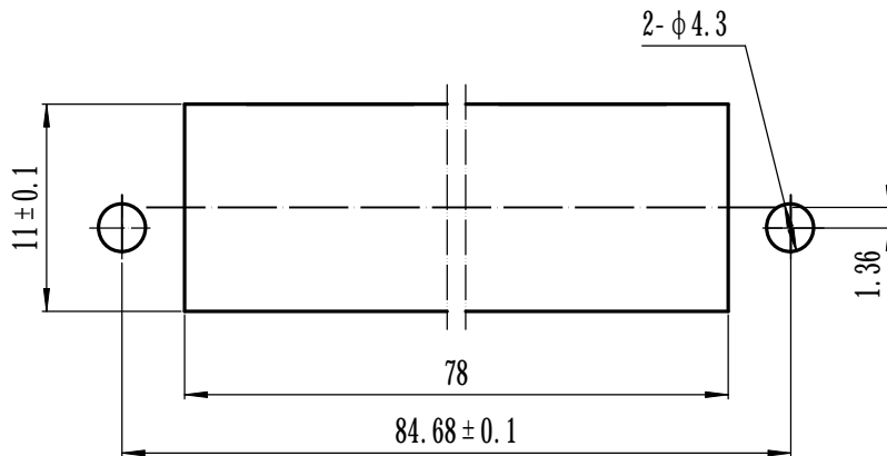
推荐插座安装开孔尺寸
