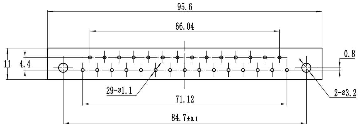
推荐插座安装开孔尺寸
