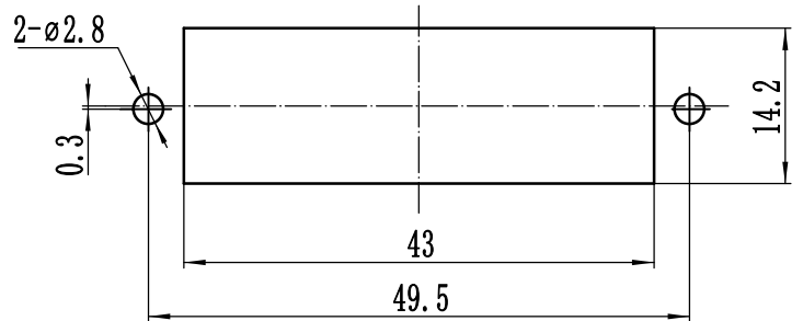
推荐插座安装开孔尺寸Z
