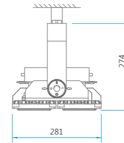
Pendant mounting bracket
