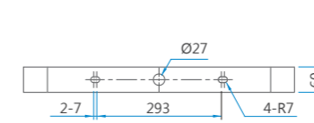
Pendant mounting bracket
