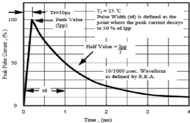
Fig. 5 - Pulse Waveform
