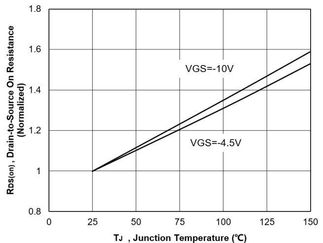
Figure 6. Normalized On-Resistance
