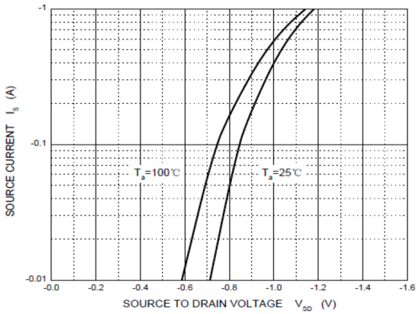
Figure 3. Diode Forward Voltage vs. current
