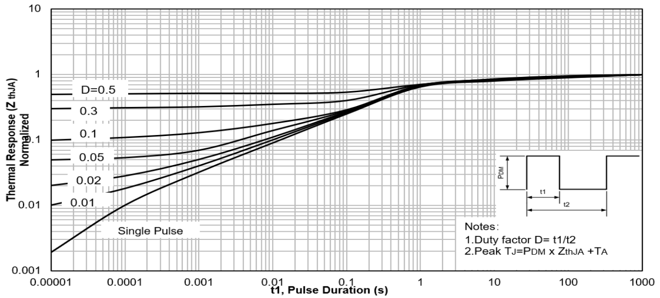
Figure 7. Maximum Effective Transient Thermal Impedance ,Junction-to-Ambient
