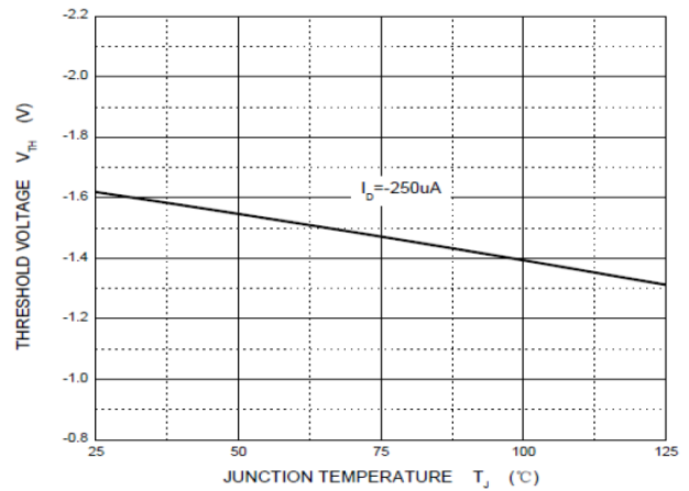
Figure 4. Gate Threshold vs. Junction Temperature
