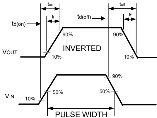
Figure 8. Switching wave
