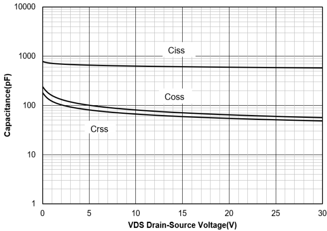
Figure 3. Capacitance Characteristics
