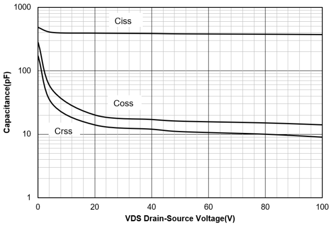
Figure 3. Capacitance Characteristics
