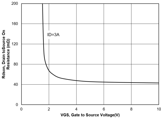
Figure 7. On-Resistance VS Gate-Source Voltage
