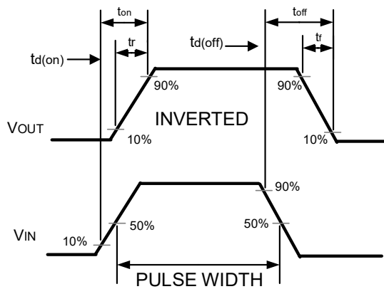
Figure 11. Switching wave
