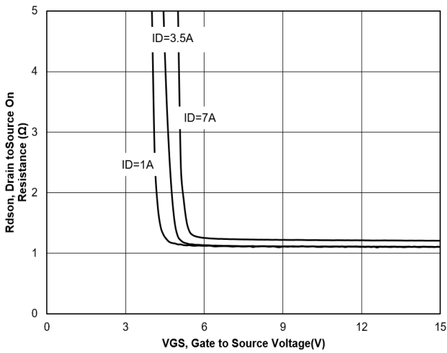
Figure 7. Typical Drain to Source ON Resistance
