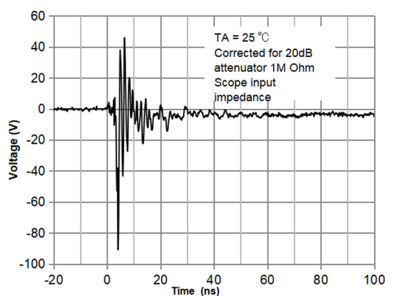
ESD Clamping Voltage(AU0971P6) -8 kV Contact per IEC61000-4-2
