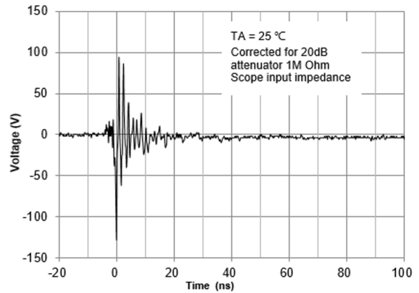
ESD Clamping Voltage(AU1271P6) -8 kV Contact per IEC61000-4-2
