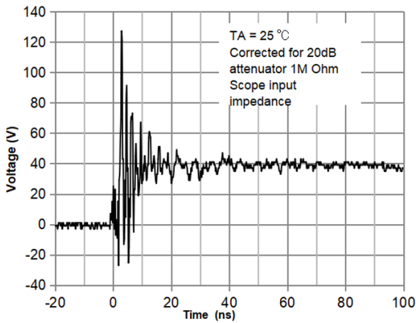
ESD Clamping Voltage(AU1571P6) 8 kV Contact per IEC61000-4-2
