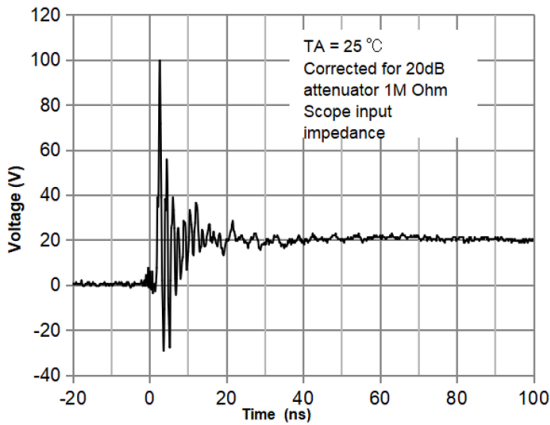
ESD Clamping Voltage(AU0571P6) 8 kV Contact per IEC61000-4-2
