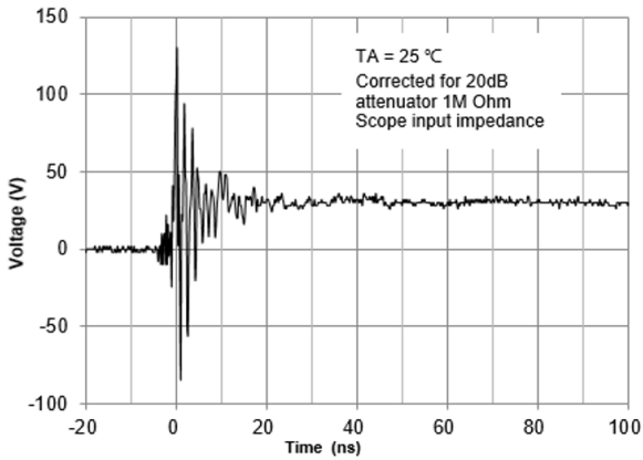
ESD Clamping Voltage(AU1271P6) 8 kV Contact per IEC61000-4-2
