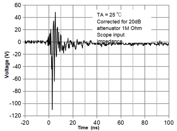
ESD Clamping Voltage(AU2471P6) -8 kV Contact per IEC61000-4-2
