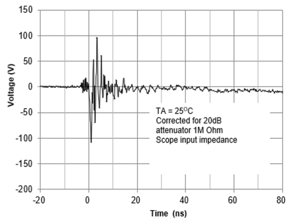
ESD Clamping Voltage(AU1871P6) -8 kV Contact per IEC61000-4-2
