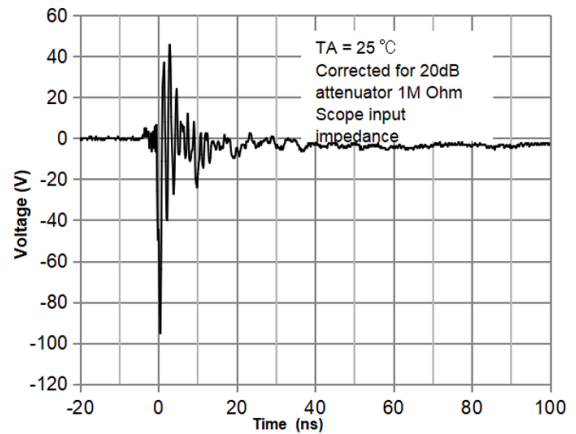
ESD Clamping Voltage(AU3671P6) -8 kV Contact per IEC61000-4-2
