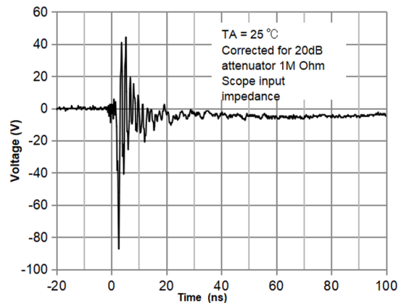
ESD Clamping Voltage(AU0571P6) -8 kV Contact per IEC61000-4-2
