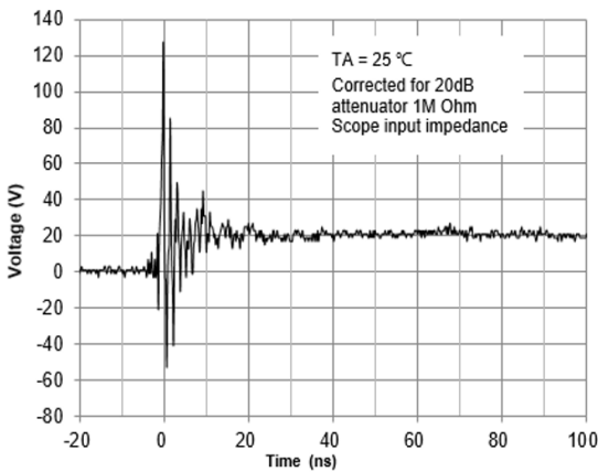
ESD Clamping Voltage(AU0771P6) 8 kV Contact per IEC61000-4-2
