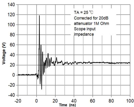
ESD Clamping Voltage(AU0971P6) 8 kV Contact per IEC61000-4-2
