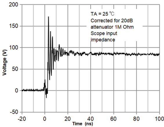
ESD Clamping Voltage(AU3671P6) 8 kV Contact per IEC61000-4-2
