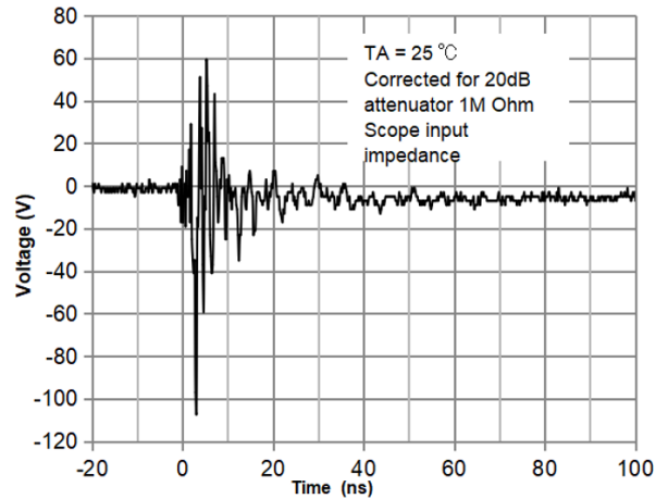
ESD Clamping Voltage(AU1571P6) -8 kV Contact per IEC61000-4-2
