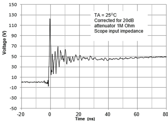
ESD Clamping Voltage(AU1871P6) 8 kV Contact per IEC61000-4-2
