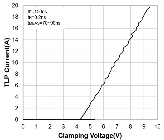
TLP Curve
