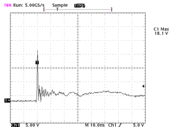
TLP Curve
