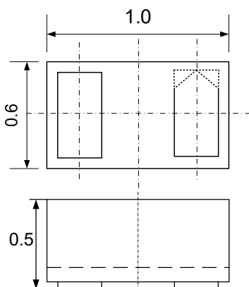
Package Dimensions
