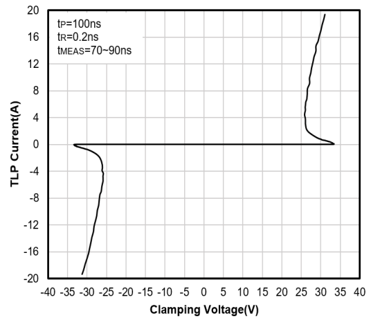
TLP Curve
