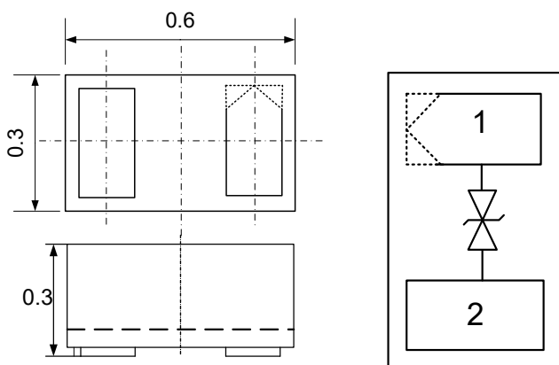
Package Dimensions
