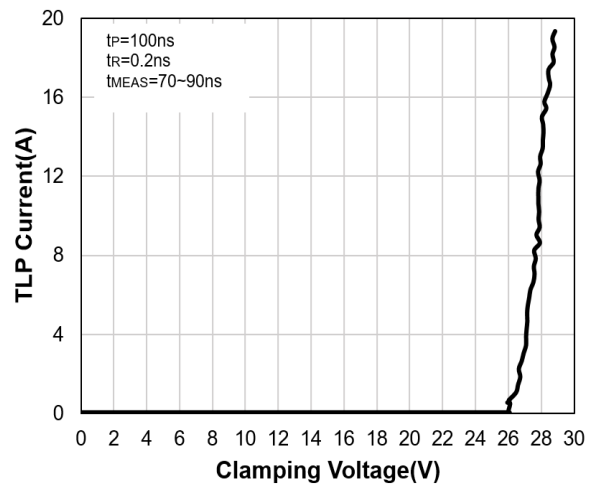
TLP Curve
