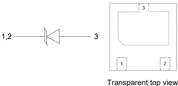
Circuit and Pin Schematic
