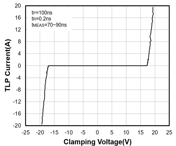
TLP Curve
