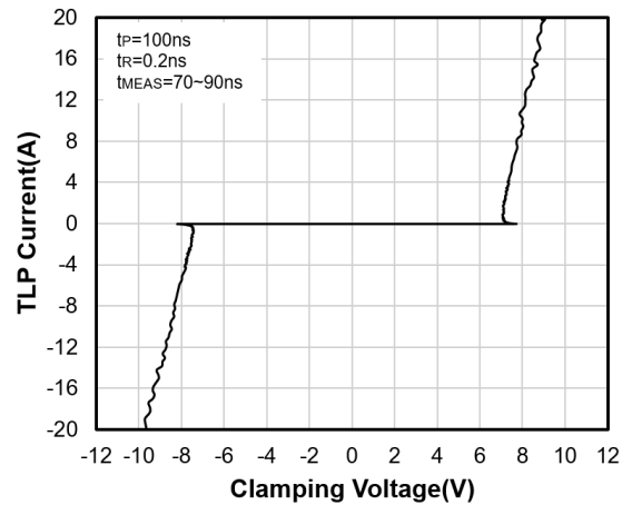
TLP Curve
