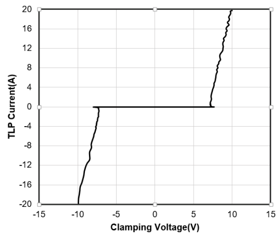
TLP Curve
