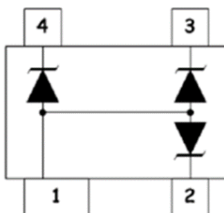
Pin Schematic
