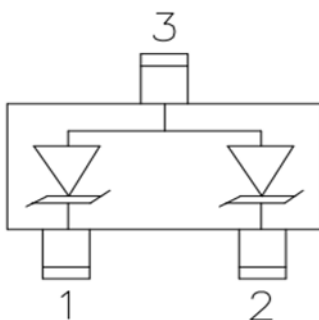
Pin Schematic
