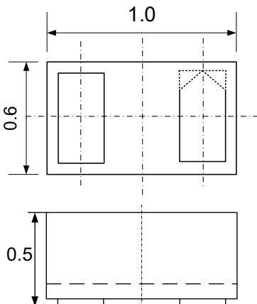
Package Dimensions
