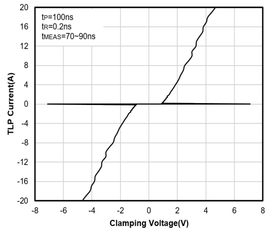
TLP Curve
