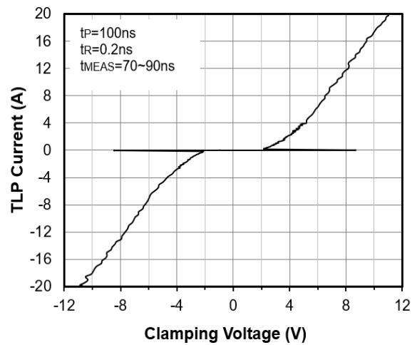
TLP Measurement
