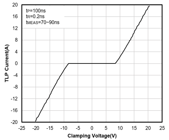
TLP Curve
