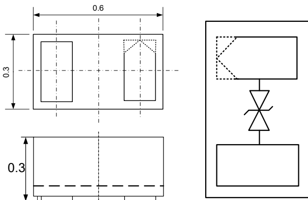
Package Dimensions
