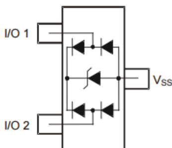
Pin Schematic
