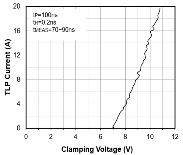
TLP Measurement
