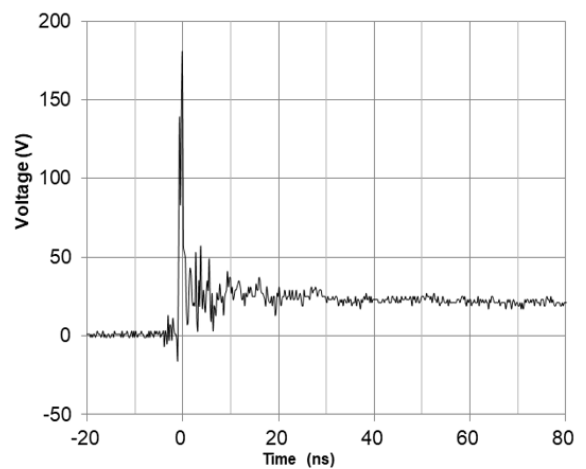
TLP Curve
