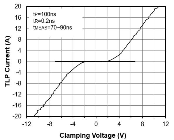
TLP Measurement
