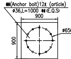
foundation (Provide by Customer)
