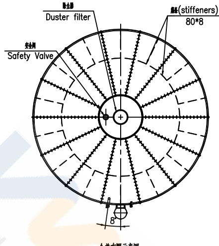
Layout of silo cover
