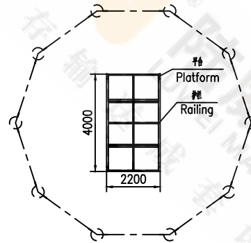
Layout of silo cover
