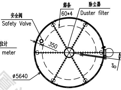
仓盖布置示意图 Layout of silo cover
