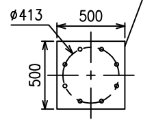
基础示意图(客户提供) foundation(Provide by Customer)
