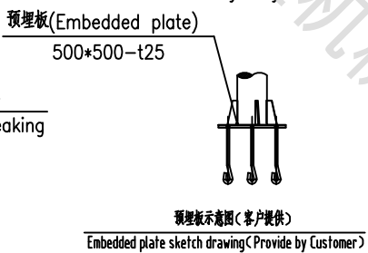
预埋板示意图(客户提供) Embedded plate sketch drawing(Provide by Customer)
