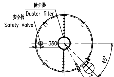
仓盖布置示意图 Layout of silo cover
