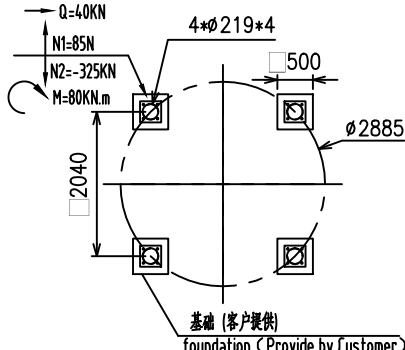
Layout of leg
