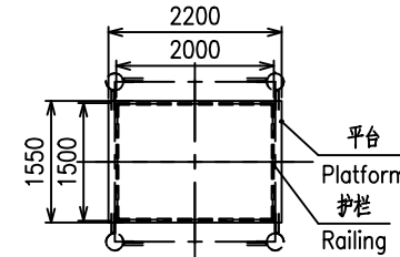
Layout of platform
