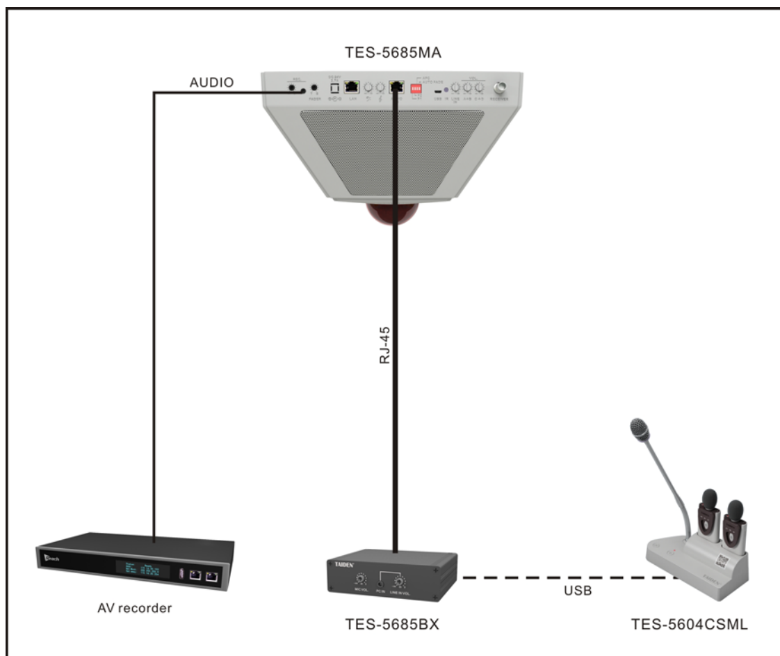
TES-5685MA Interactive Audio Recording System Solution
